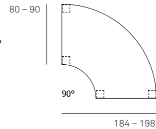
640/11 System panels Extension leaf Arc-shaped module 90°
