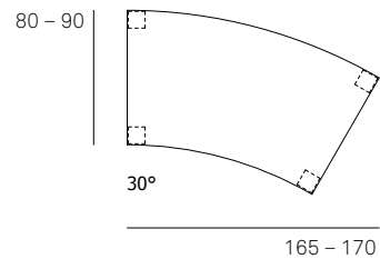
640/11 System panels Extension leaf Arc-shaped module 30°
